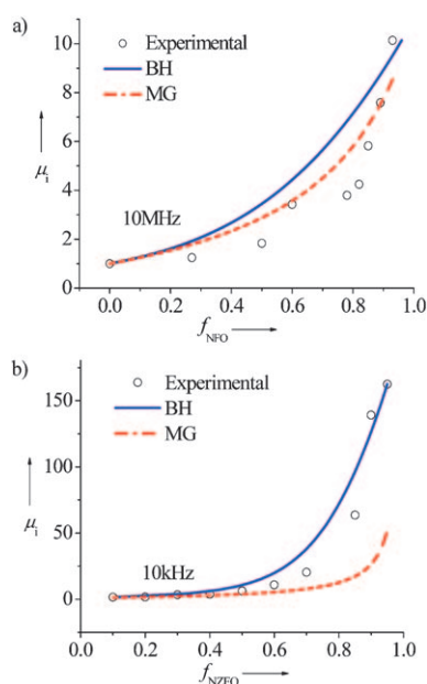
Figure 4. Variation of the initial permeability ( \mu_i ) of a) PTO/NFO and b) BTO/NZFO ceramic composites with ferrite volume fraction at applied frequency of 10 MHz and 10 kHz, respectively. Also shown are the calculated lines from the Maxwell–Garnett (MG) and Bruggeman–Hanai (BH) equations (see the Supporting Information).
